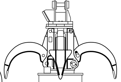
(b) Electrohydraulic Grapple
