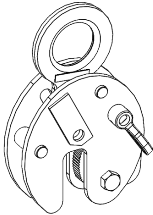
(a) Plate Clamp
