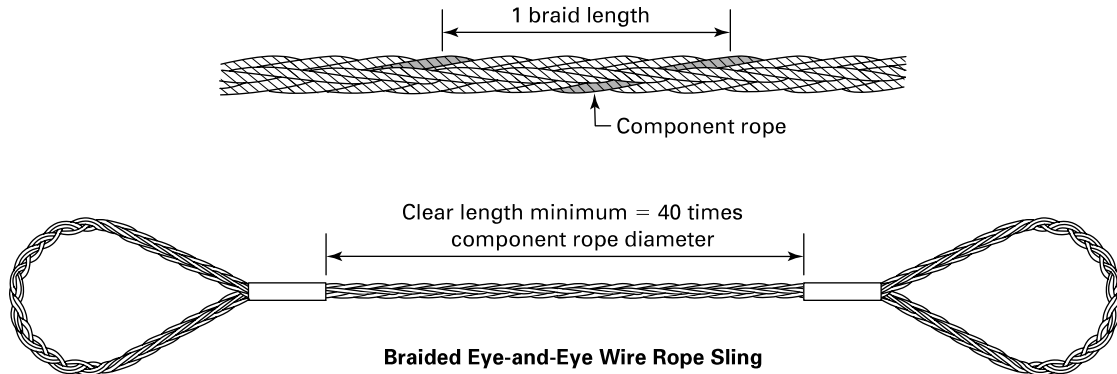
Figure 9-2.3.2-2 Minimum Braided Slings Length
