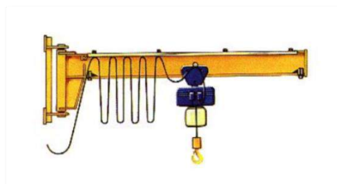
Wall/ column underbraced slewing jib crane – note the position of the stops
