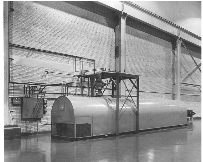
FIGURE A.4.6.6 A Typical Low-Pressure Storage Facility.
