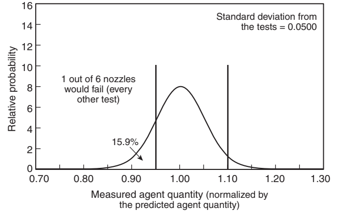
FIGURE A.5.5.3.2(g) Distribution Curve No. 6.
