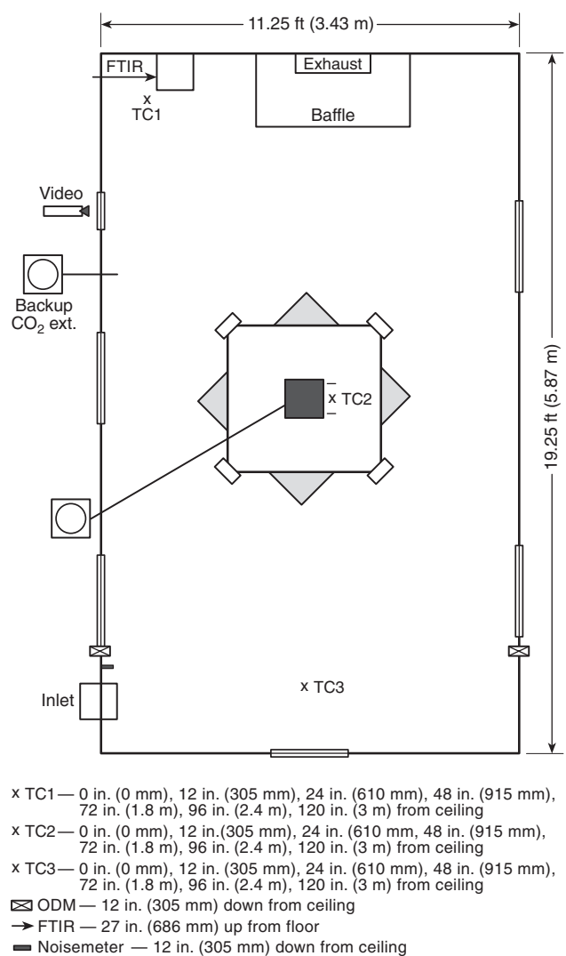
FIGURE A.5.4.2.2(b) Chamber Plan View.
