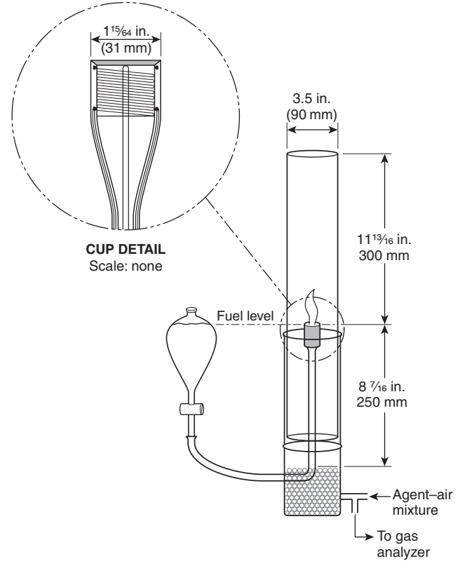
FIGURE B.19(a) Cup Burner Apparatus.
