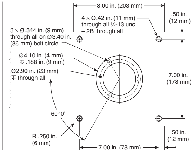
FIGURE B.19(g) Base Support Plate, \frac{3}{8} in. Thick.
