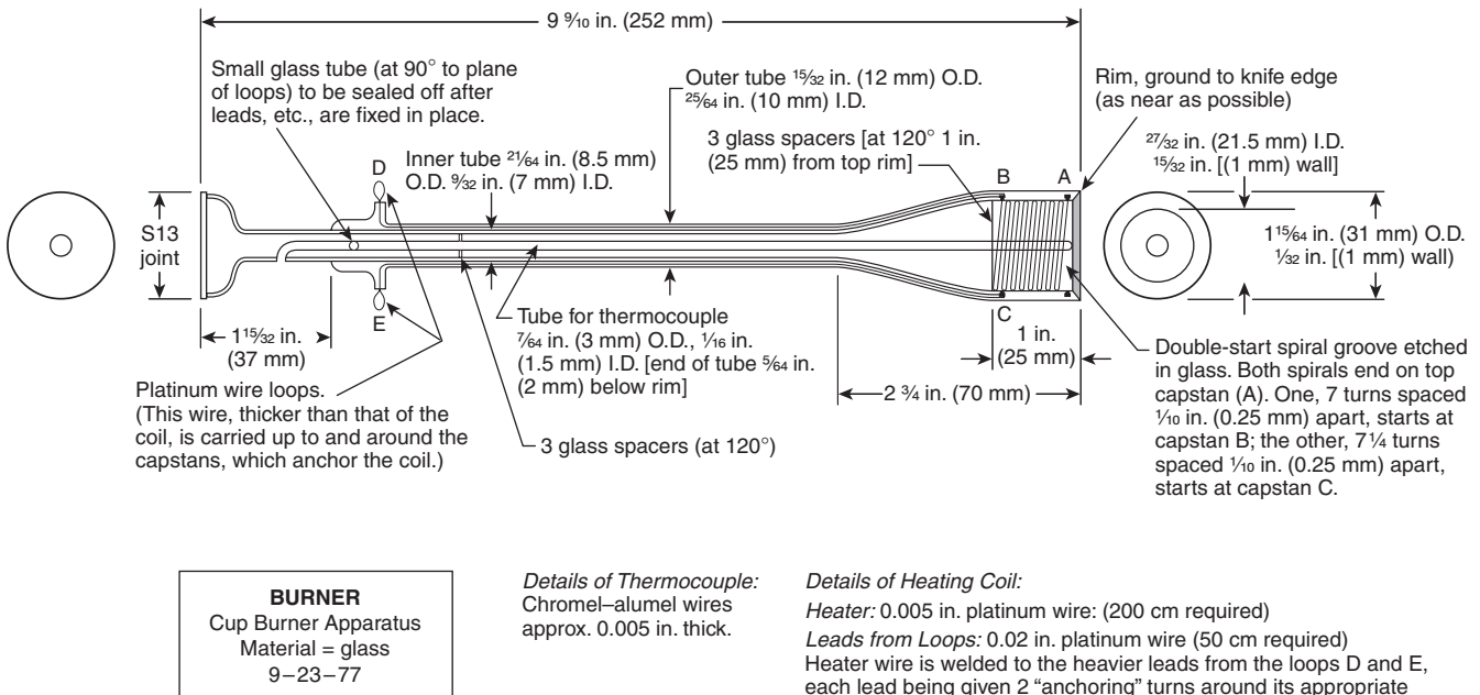
FIGURE B.19(b) Details of Cup Design. Used by Permission of ICI.
