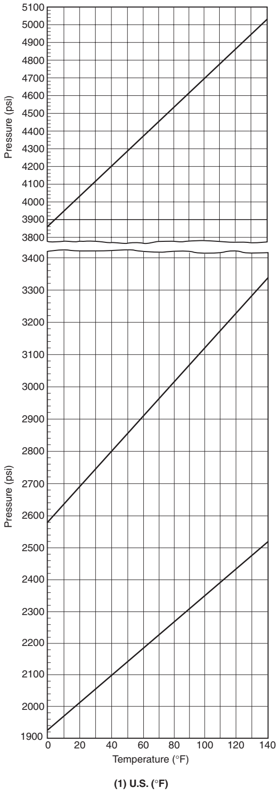
FIGURE A.4.1.4.1(l) Isometric Diagram of IG-55.
