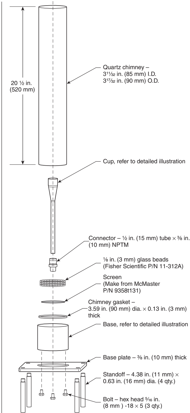
FIGURE B.19(c) Cup Burner Assembly (Exploded View).
