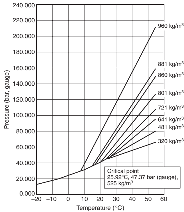
FIGURE A.4.1.4.1(g) Isometric Diagram of HFC-23.
