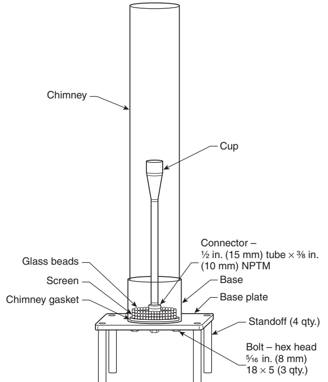
FIGURE B.19(d) Cup Burner Assembly (Transparent View).
