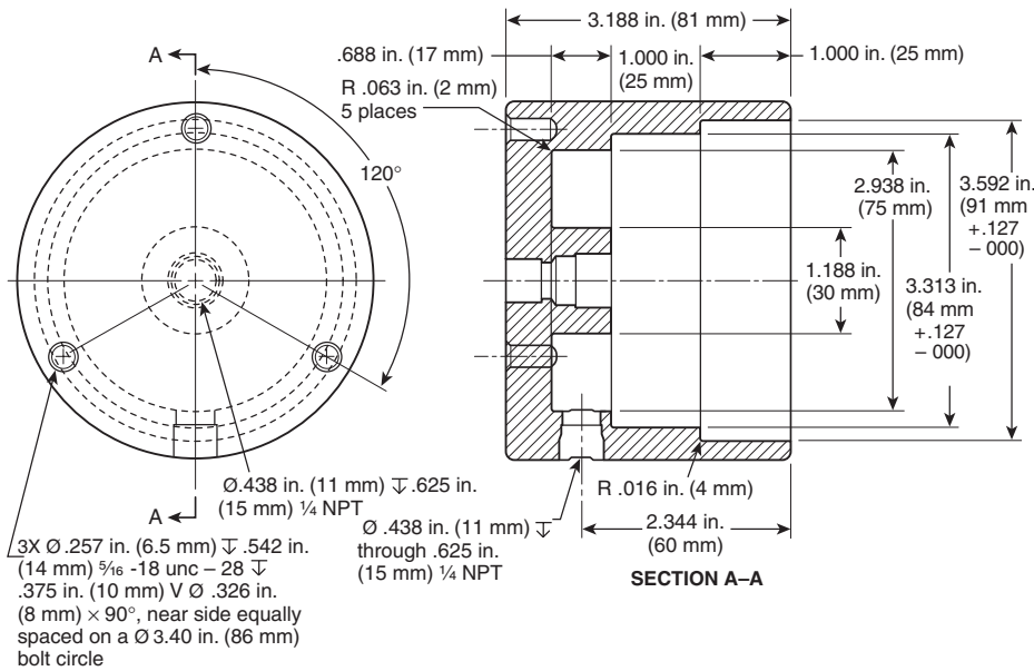
FIGURE B.19(e) Cup Material: Quartz [Dimension in Inches (mm in brackets)].
