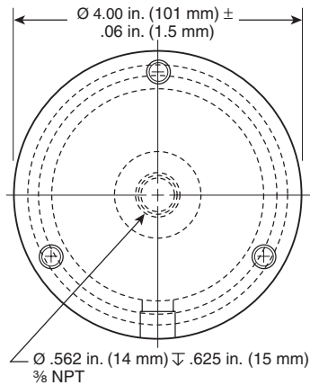
FIGURE B.19(f) Base, Detail.
