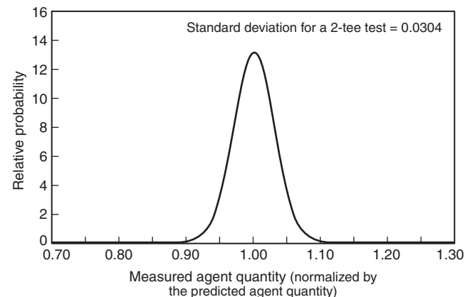
FIGURE A.5.5.3.2(a) Normal Distribution Curve.
