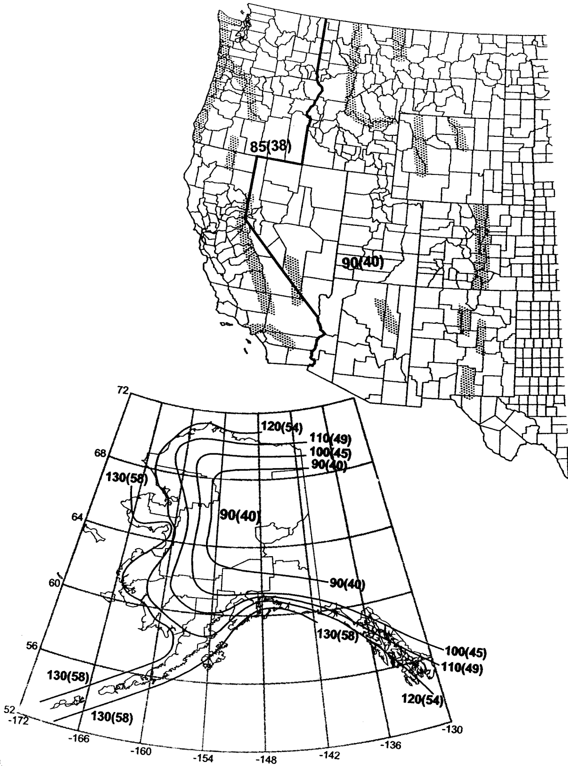
FIGURE A.35.9.2.2(c) Basic Wind Speed. (Source: Reprinted with permission from ASCE/SEI 7.)
