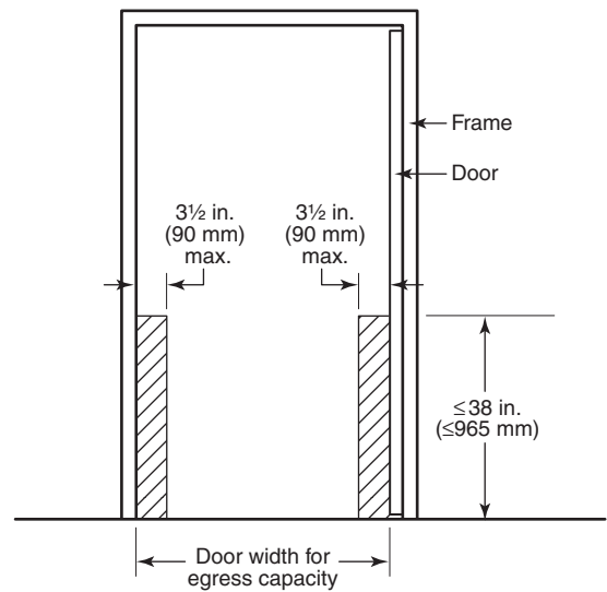
FIGURE A.11.2.1.2.2(b) Door Width — Egress Capacity with Permitted Obstructions.
