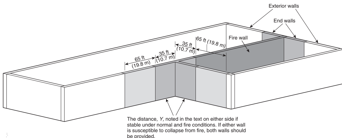
FIGURE 8.3.2.16.3.1 Angle Wall Exposure Protection. [221: Figure 5.16.3.1]
