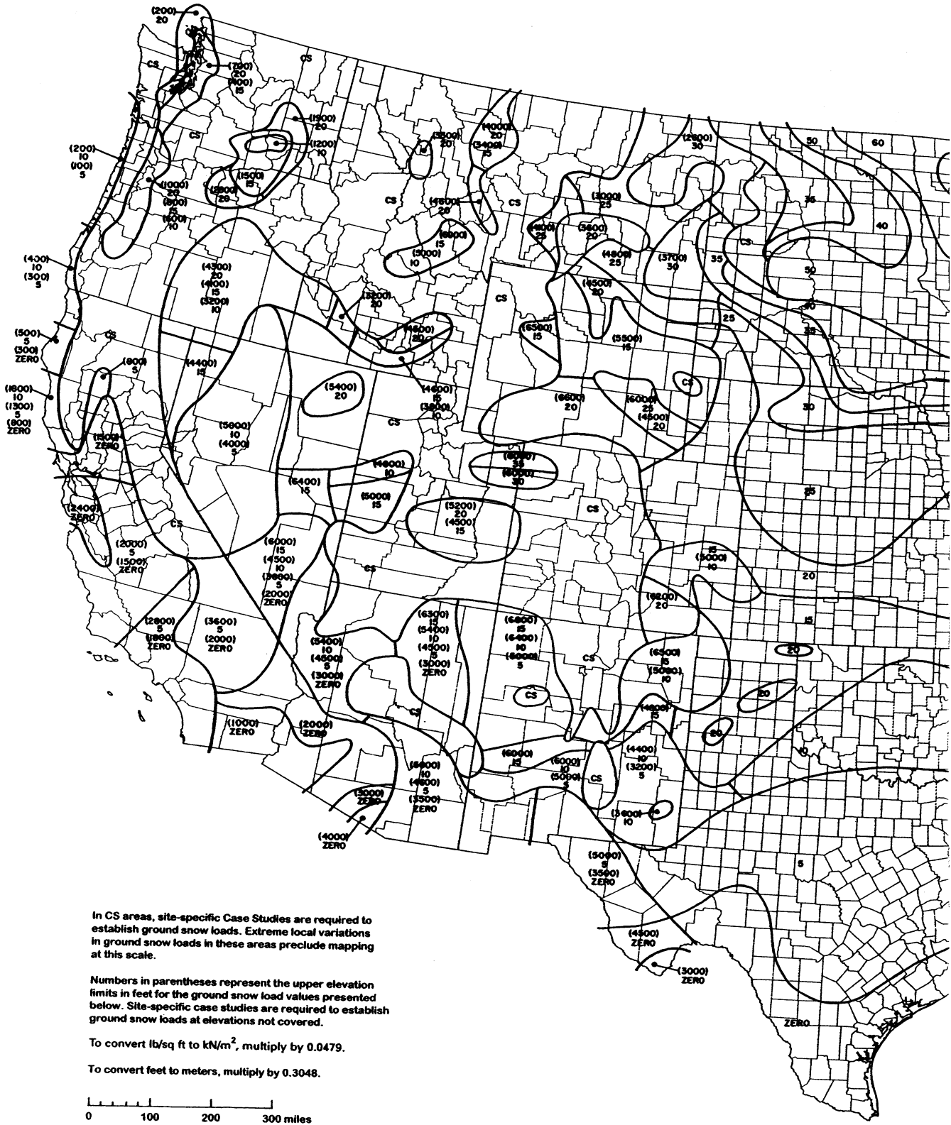
FIGURE A.35.8.2 Ground Snow Loads, p_g , for the United States (lb/ft 2 ). (Source: Reprinted with permission from ASCE/SEI 7.)
