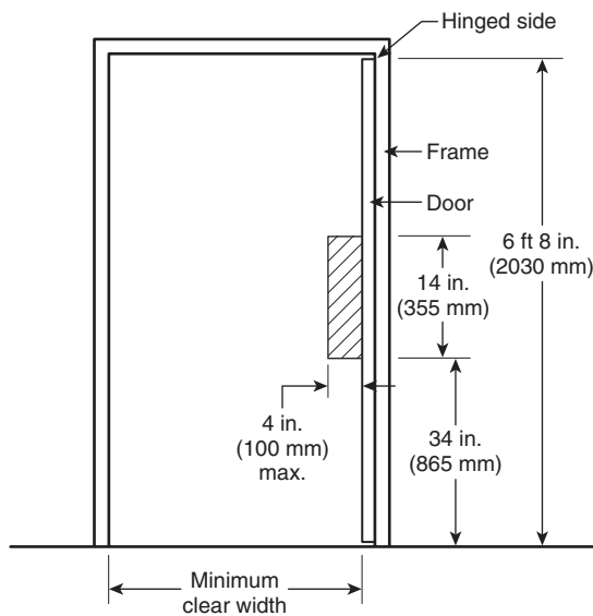
FIGURE A.11.2.1.2.1(b) Minimum Clear Width with Permitted Obstructions.
