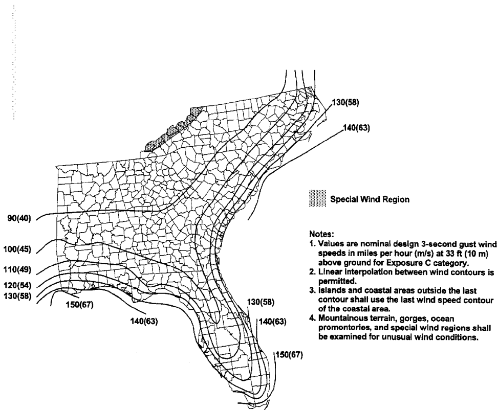
FIGURE A.35.9.2.2(b) Basic Wind Speed — Gulf of Mexico Southeastern U.S. Hurricane Coastline. (Source: Reprinted with permission from ASCE/SEI 7.)
