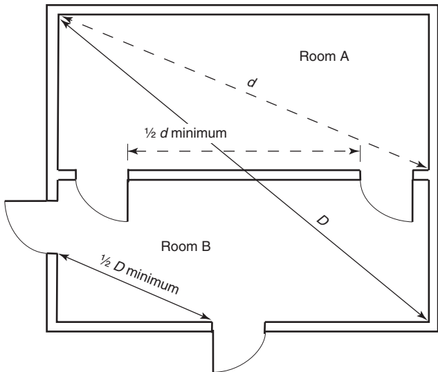
FIGURE A.11.5.1.4.2(b) Diagonal Rule for Exit and Exit Access Door Remoteness.
