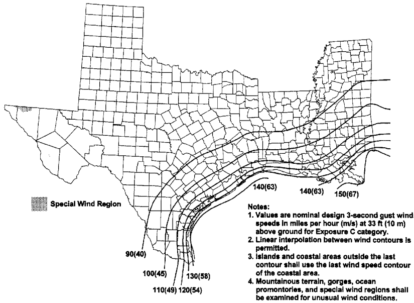
FIGURE A.35.9.2.2(a) Basic Wind Speed — Gulf of Mexico Hurricane Coastline. (Source: Reprinted with permission from ASCE/SEI 7.)
