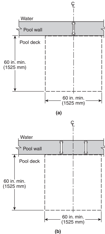
FIGURE 12.45.15.4.1 Clear Deck Space at Transfer Walls. [ADA/ABA-AG: Figure 1009.4.1]
