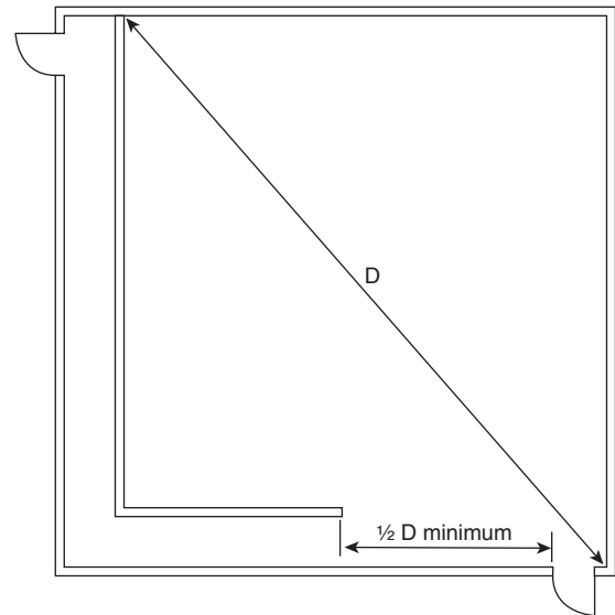
FIGURE A.11.5.1.4.2(c) Diagonal Rule for Exit and Exit Access Remoteness.
