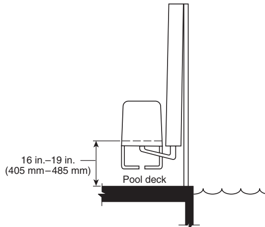
FIGURE 12.45.15.2.4 Pool Lift Seat Height. [ADA/ABA-AG: Figure 1009.2.4]
