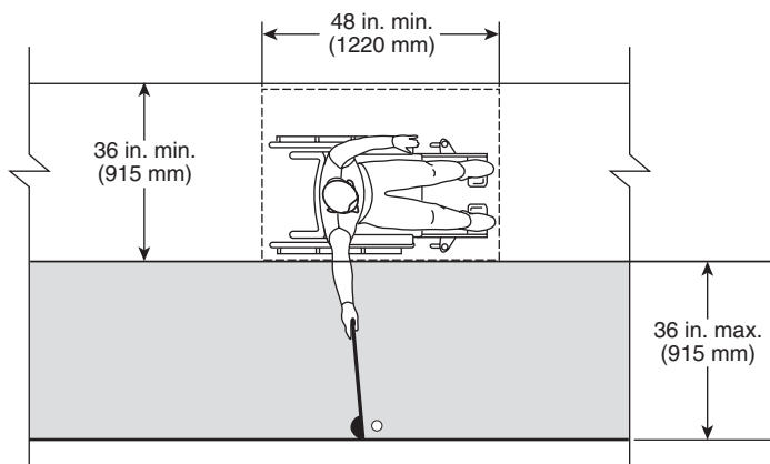
FIGURE 12.45.13.3.2 Golf Club Reach Range Area. [ADA/ABA-AG: Figure 1007.3.2]
