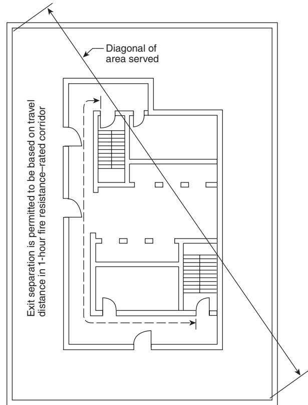
FIGURE A.11.5.1.4.4 Exit Separation Measured Along Corridor Path.
