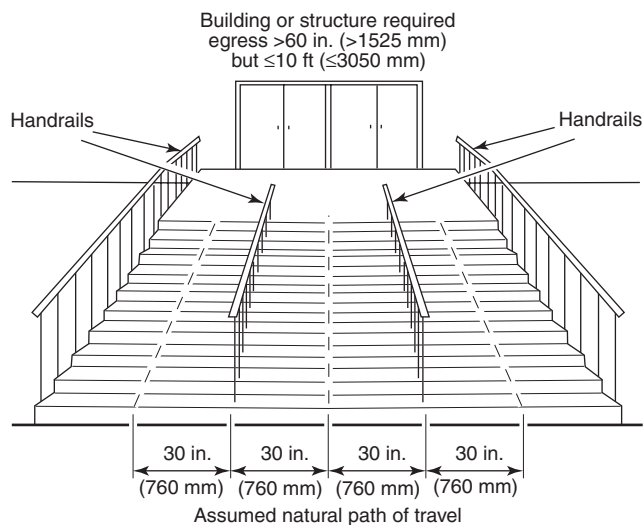
FIGURE A.11.2.2.4.2 Assumed Natural Paths of Travel on Monumental Stairs with Various Handrail Locations.
