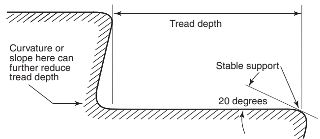
FIGURE A.11.2.2.3.5(d) Tread Measurement with Stable Support at Leading Edge.
