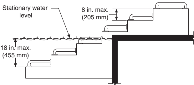
FIGURE 12.45.15.5.4 Transfer Steps. [ADA/ABA-AG: Figure 1009.5.4]
