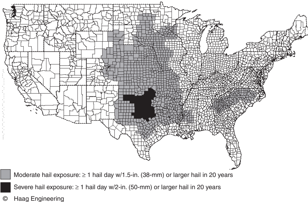
FIGURE 38.5.1 Hail Exposure Map. ©Haag Engineering
