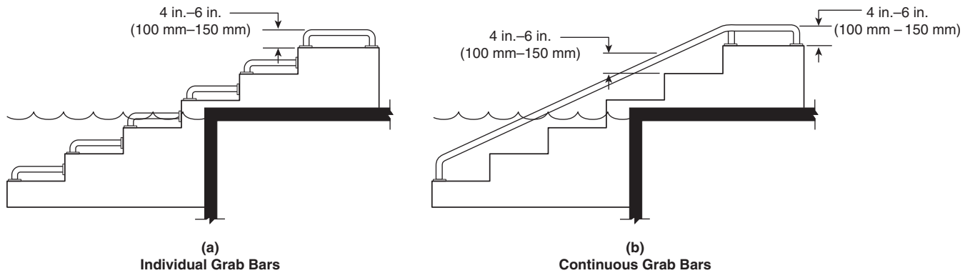
FIGURE 12.45.15.5.7 Grab Bars. [ADA/ABA-AG: Figure 1009.5.7]
