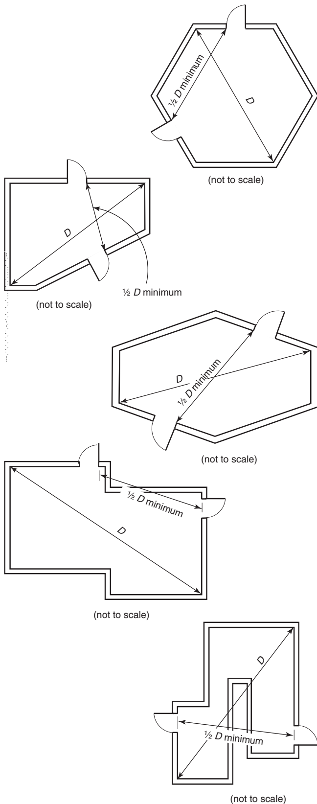
FIGURE A.11.5.1.4.2(e) Diagonal Measurement for Unusually Shaped Areas.
