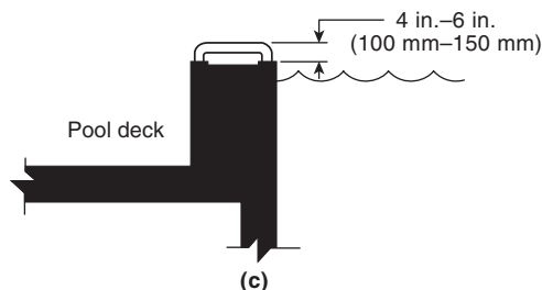
FIGURE 12.45.15.4.5 Grab Bars for Transfer Walls. [ADA/ABA-AG: Figure 1009.4.5]
