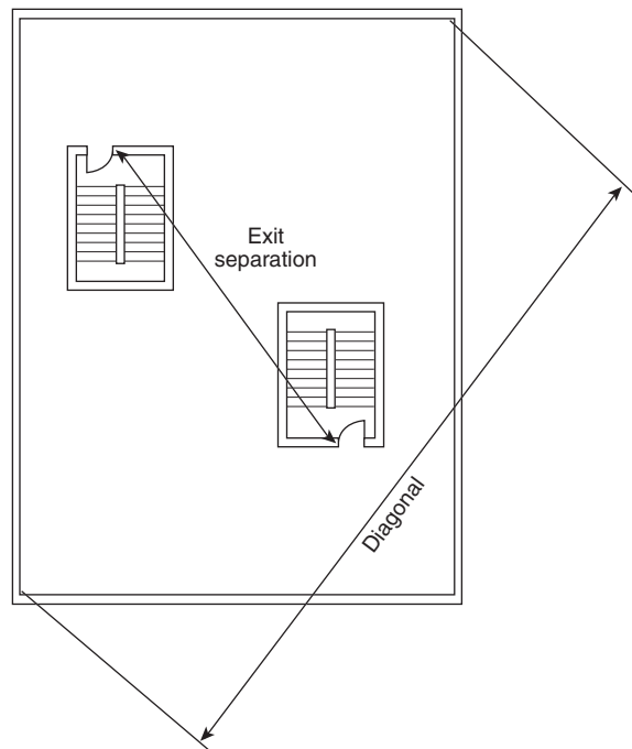
FIGURE A.11.5.1.4.2(d) Exit Separation and Diagonal Measurement of Area Served.
