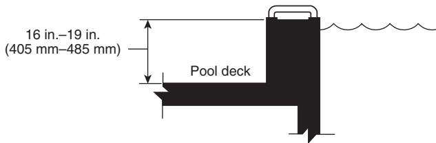
FIGURE 12.45.15.4.2 Transfer Wall Height. [ADA/ABA-AG: Figure 1009.4.2]
