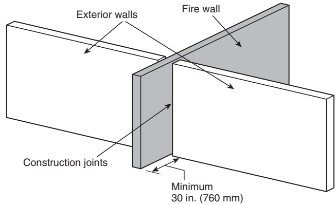
FIGURE 8.3.2.16.2.3 End Wall Exposure Protection for Light Hazard and Ordinary Hazard (Group 1 or Group 2) Occupancies. [221: Figure 5.16.2.3]
