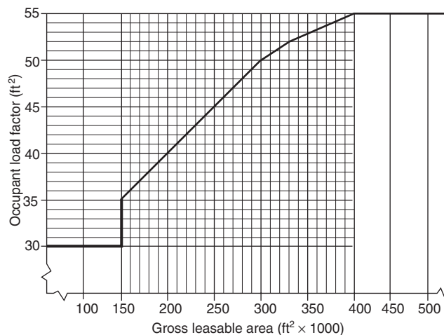
FIGURE 11.3.1.2 Mall Building Occupant Load Factors.
