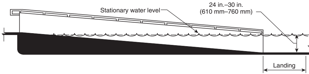
FIGURE 12.45.15.3 Sloped Entry Submerged Depth. [ADA/ABA-AG: Figure 1009.3.2]
