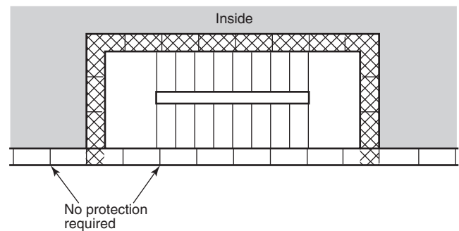
FIGURE A.11.2.2.5.2(a) Stairway with Nonrated Exterior Wall in Same Plane as Building Exterior Wall.
