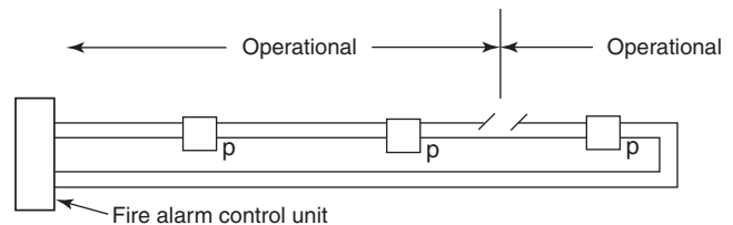
FIGURE G.2.2 Nonpowered Alarm-Initiating or Supervisory-Initiating Devices Connected to Style D or E Initiating Device Circuits.
