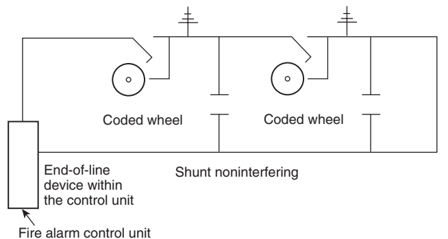
FIGURE G.3.10 Style 4.5 (Class B).
