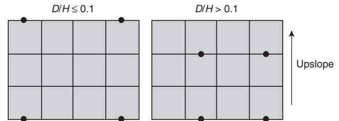
FIGURE A.17.7.3.2.4.5 Spot-Type Detector Spacing for Sloping Ceilings with Beam Pockets.
