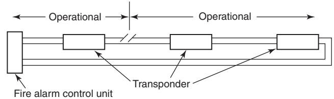
FIGURE G.3.14(a) Style 7.0 (Class A).
