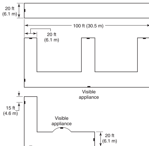
FIGURE A.18.5.4.4 Corridor Spacing for Visible Appliances.
