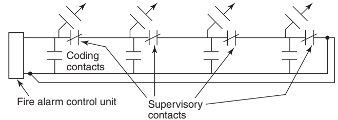
FIGURE G.3.3 Style 0.5(b) (Class B) Shunt.
