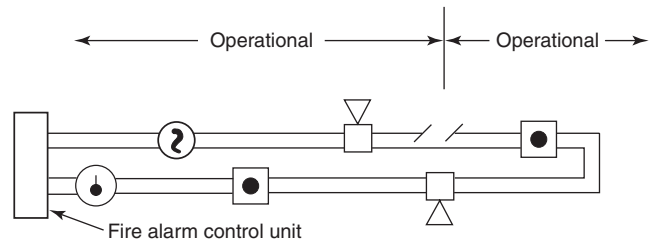
FIGURE G.2.6 Combination Alarm-Initiating Device and Notification Appliance Circuits Arranged for Operation with a Single Open or Ground Fault.
