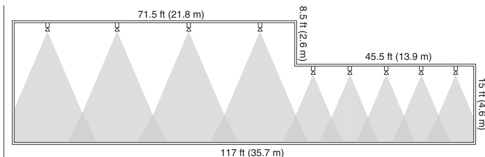
FIGURE D.2.3.1.7 Illustration Demonstrating the Effect of Ceiling Height. (Source: R. P. Schifiliti Associates, Inc.)
