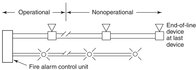
FIGURE G.2.11 Supervised Audible Notification Appliance Circuit and an Unsupervised Visible Notification Appliance Circuit.
