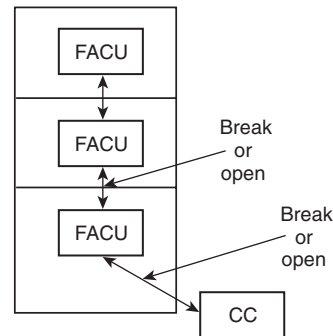
FIGURE G.3.14(g) Style 4 Fiber Network (Single Break).
