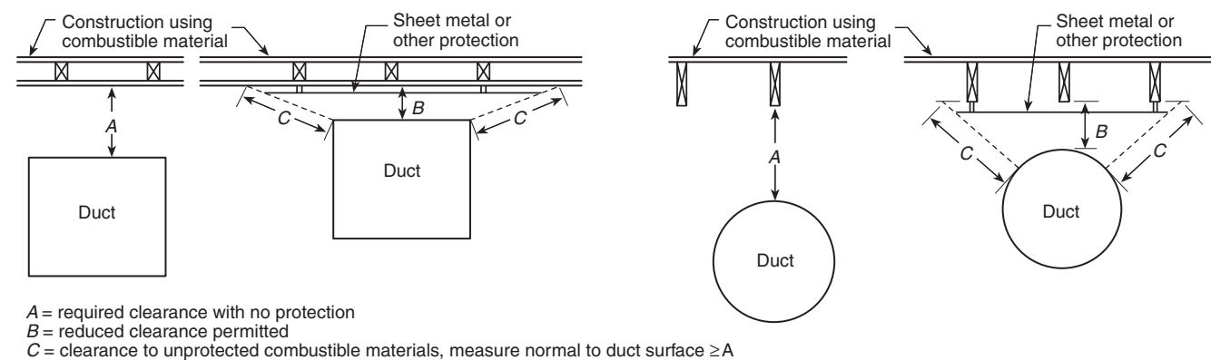
FIGURE 4.6.5.1 Extent of Protection Required to Reduce Clearances from Ducts.
