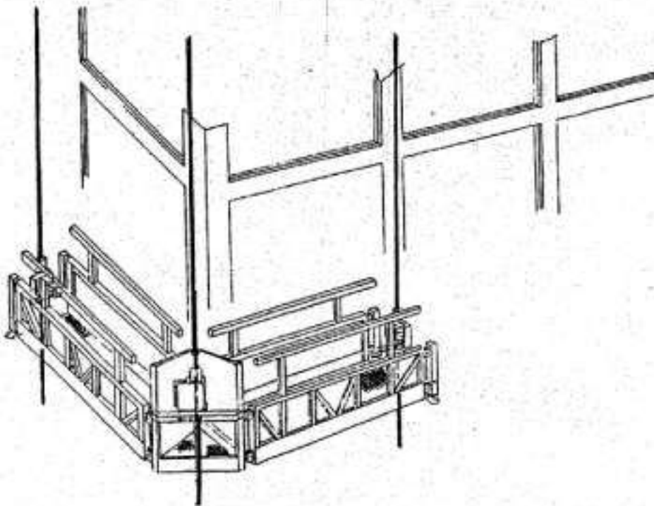
Modular Suspended Scaffold with an Angled Section
