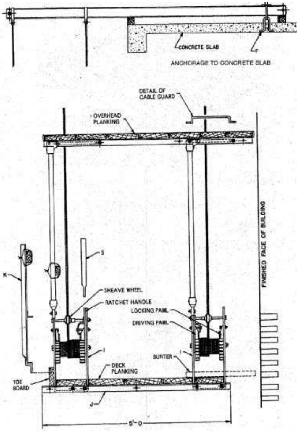
Masons' Adjustable Multiple-Point Suspension Scaffold
