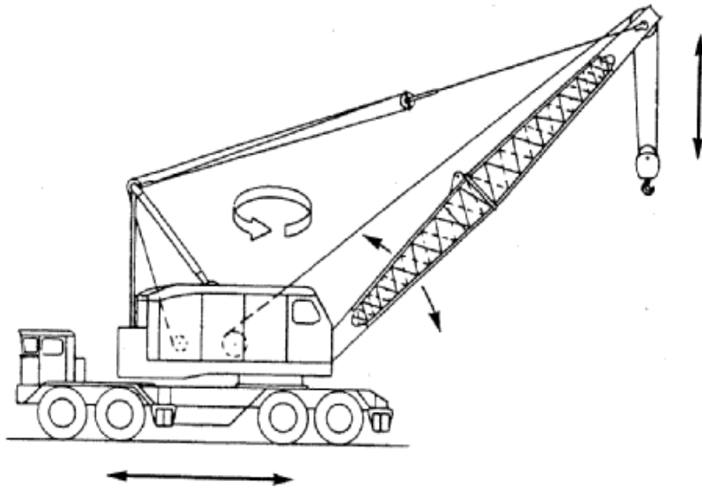
WHEEL-MOUNTED CRANE (MULTIPLE CONTROL STATION)
