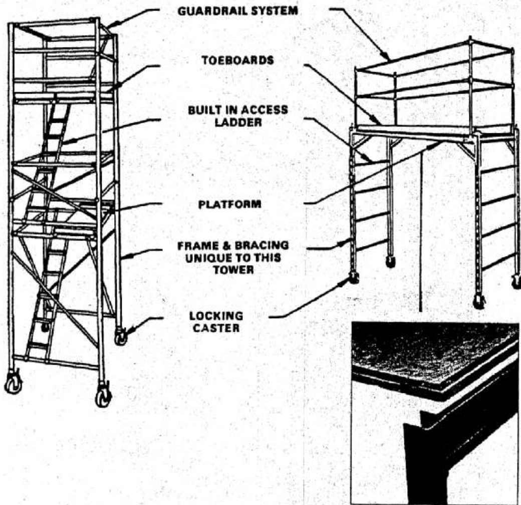
Truss and Platform
