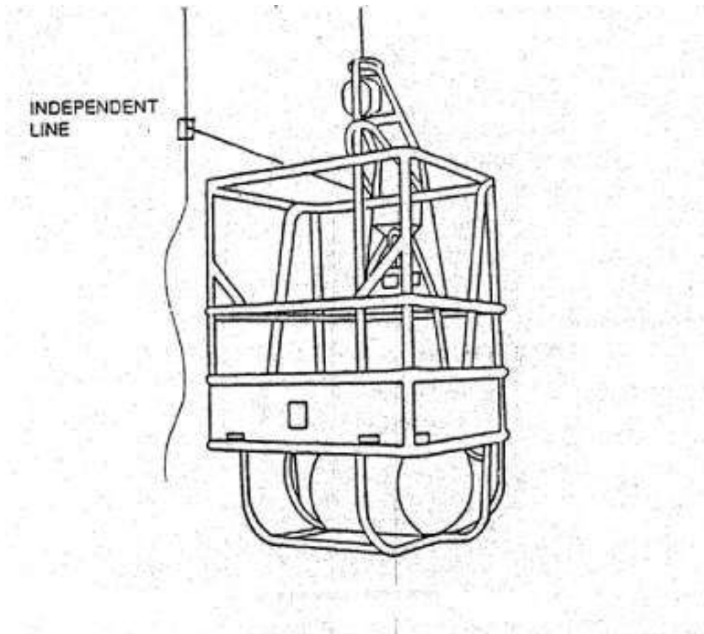
Single-Point Suspension Scaffold with Winding Drum Hoist
